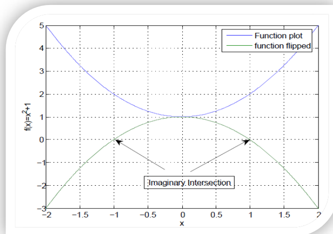
1 Figure 1 Geometric representation of imaginary roots of x^2 + 1 = 0
