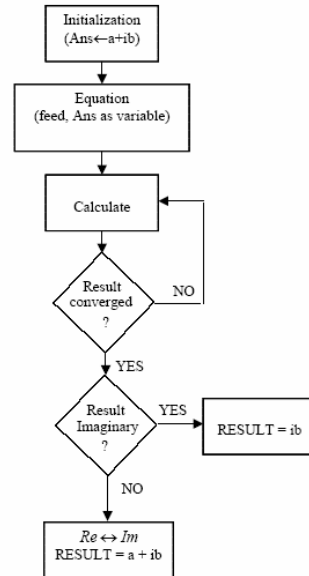
Figure 2 Flowchart of computational procedure for finding complex roots 2
