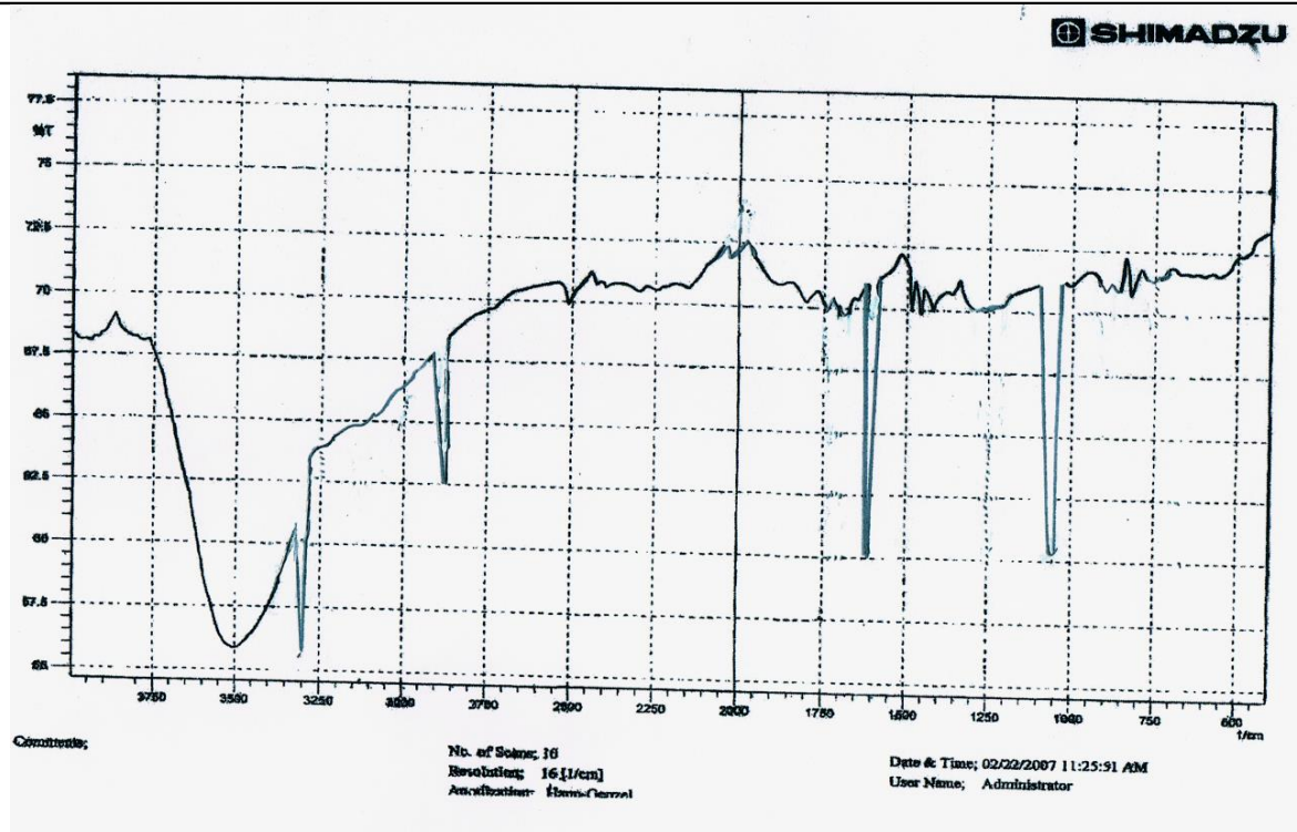
Figure -2: The FT – IR spectrum of the prepared copolymer .
