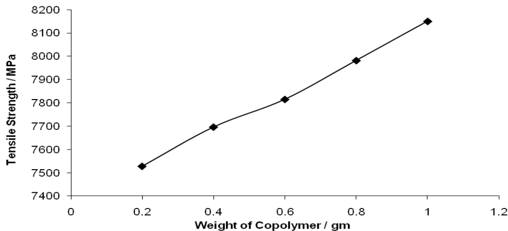
Figure - 6 : The influence of different weight of the copolymer on tensile strength of specimens .
