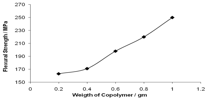
Figure - 5 : The influence of different weight of the copolymer on flexural strength of specimens .
