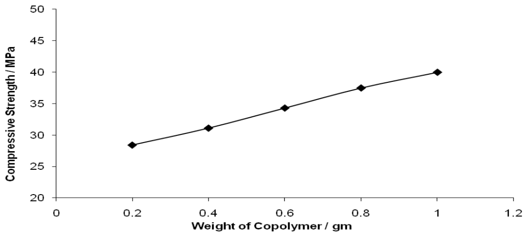
Figure - 4 : The influence of different weight of the copolymer on compressive strength of specimens .
