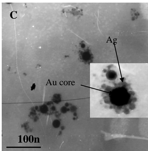
Fig. (4) TEM images and size distributions of the (A) silver, (B) gold, (C) composite nanoparticles, produced by laser ablation of target plate immersed in DDDW.
