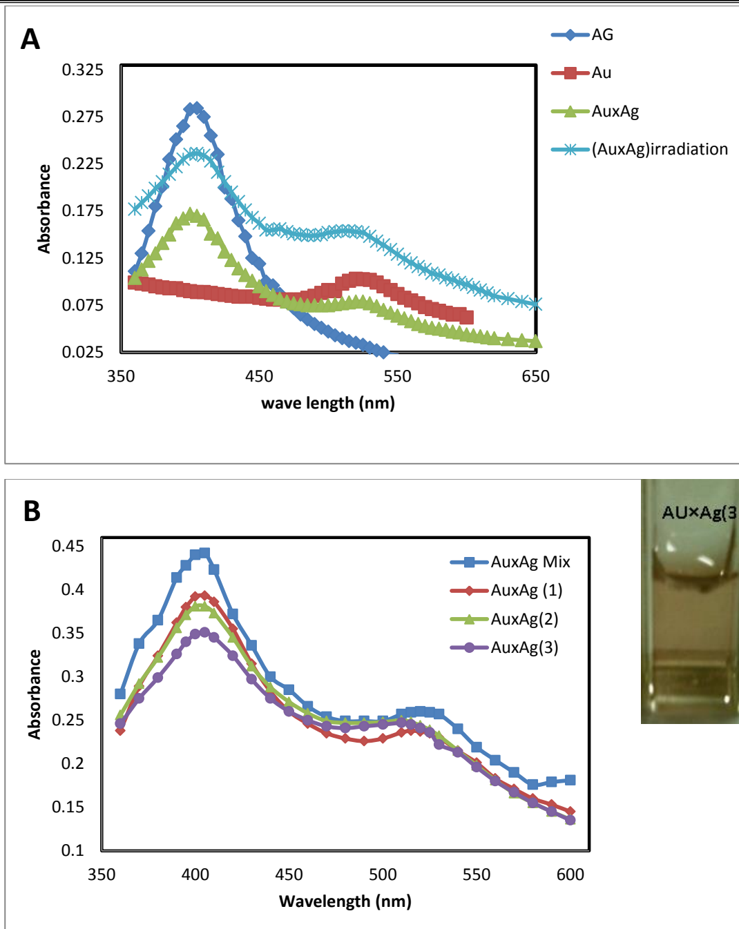
Fig. (3) Plasmon resonance spectra of (A) pure Ag NPs, Au NPs, mixture of Au/Ag NPs and irradiated Au/Ag NPs mixture ( \lambda=532 nm, laser shots of 100 pulses and E=700 mJ). (B) The effect of laser shoots (100 pulses, 700Mj each step) on Au/Ag core-shell absorption peaks.
