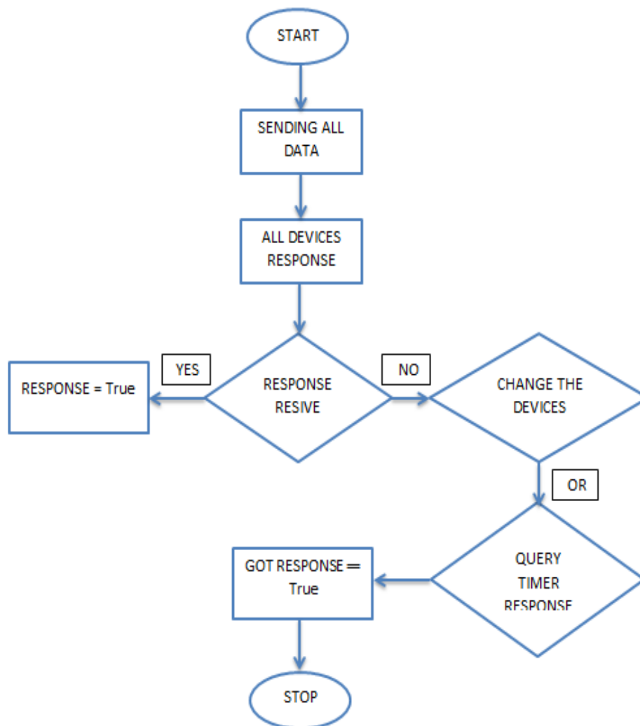
Figure ٦: Flow Chart to Disable or stop the devices
