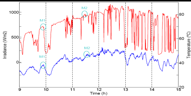
Fig.(18)Irradiance and module temperature measured in April 2012
