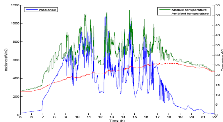
Fig.(13)The effect of irradiance and ambient temperature on the calculated module temperature.
