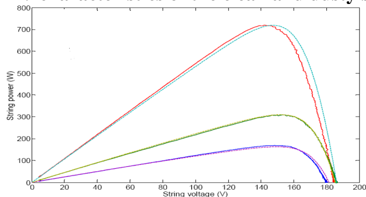
Fig.(23) The P-V characteristics of the clean and dusty solar cells in September 2011.
