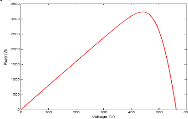
Fig.(12)P-V characteristics of the solar cells used
