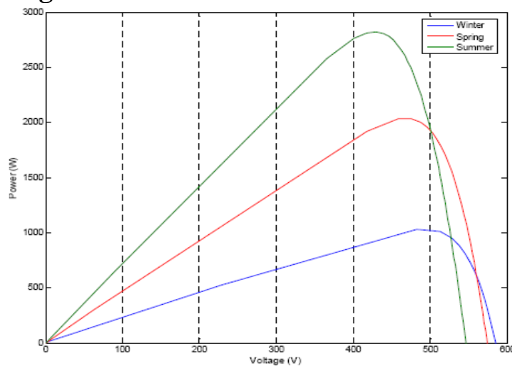
Fig.(15) The P-V performance characteristics of the clean solar cells during winter, spring and summer.
