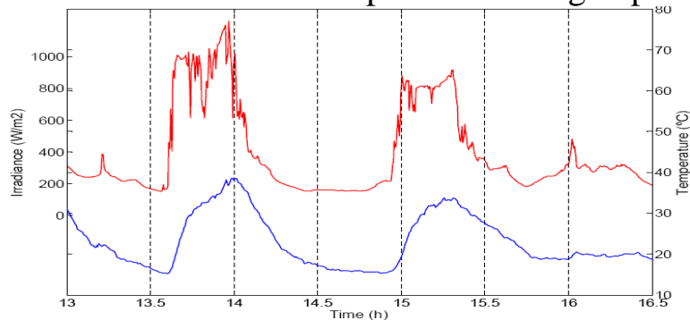
Fig.(19)Irradiance and module temperature measured in September 2011
