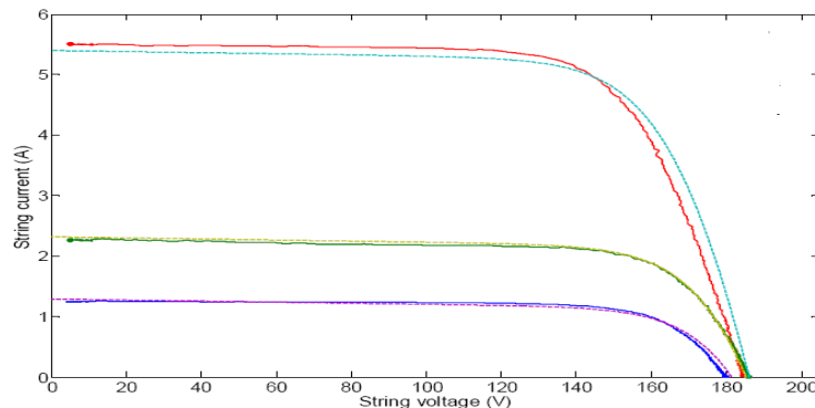
Fig.(22)The I-V characteristics of the clean and dusty solar cells
