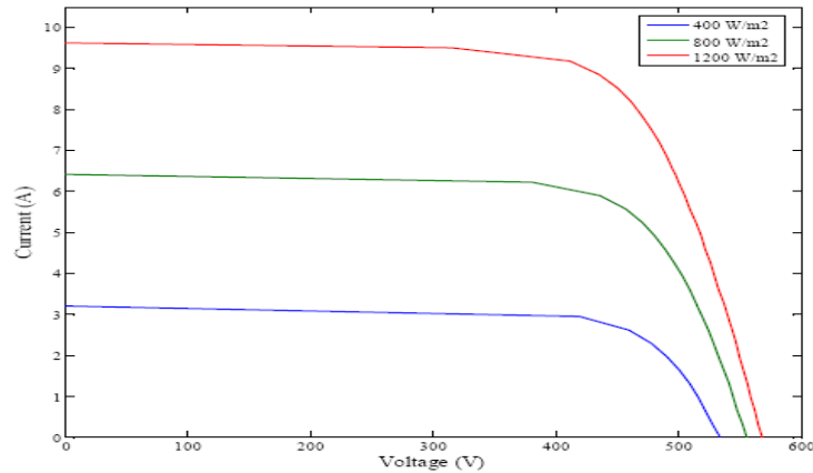
Fig.(8)The effect of irradiance on the I-V characteristics of a PV module
