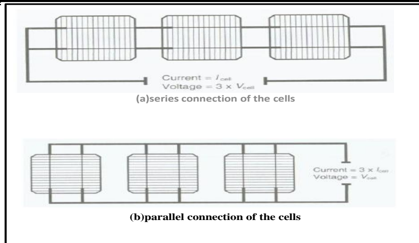
Fig.(1) Types of cell connections
