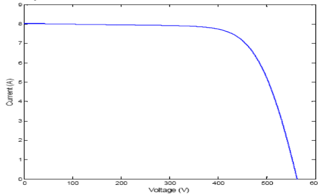
Fig.(11)I-V characteristics of the solar cells
