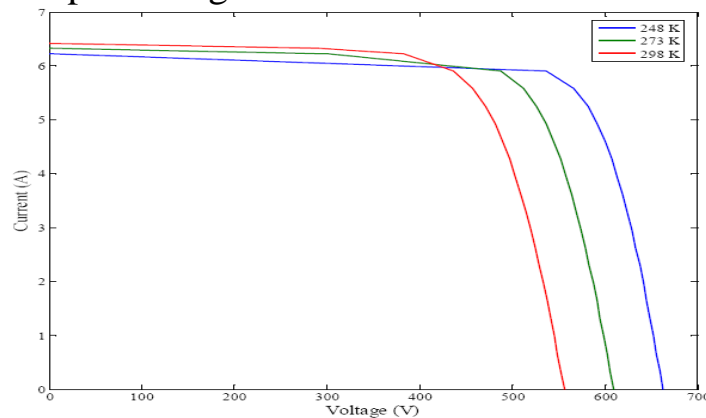
Fig.(9)The effect of temperature on the I-V characteristics of a PV module with irradiance of 800 w/m 2
