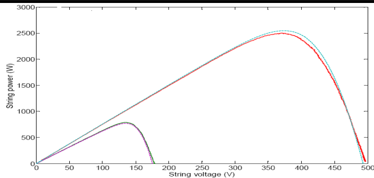
Fig.(21)The P-V characteristics of the clean and dusty solar cells
