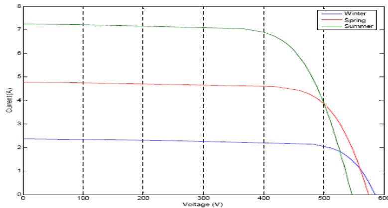
Fig.(14)The I-V performance characteristics of the clean solar cells in winter, spring and summer
