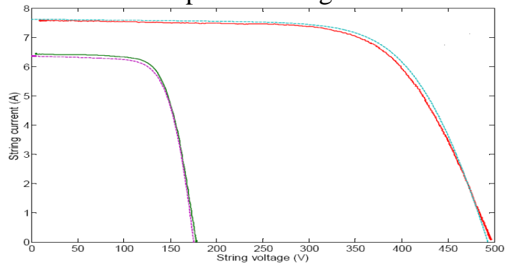
Fig.(20)The I-V characteristics of the clean and dusty solar cells
