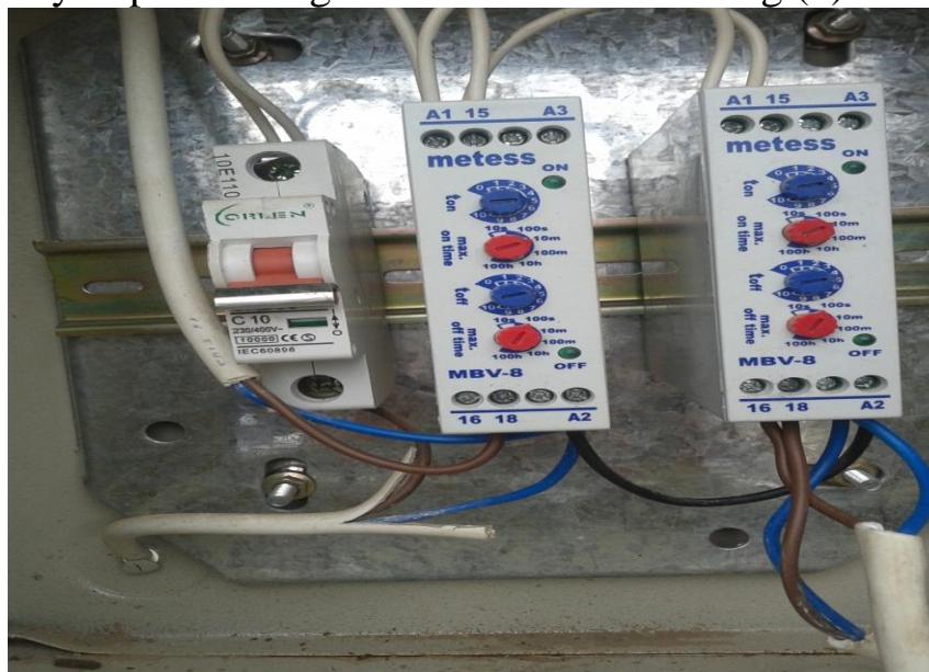
Figure(7) Control timing system
