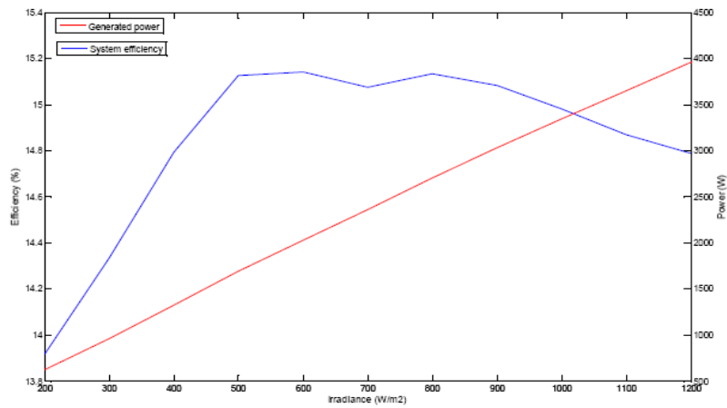
Fig.(17)The efficiency and power generated against the irradiance
