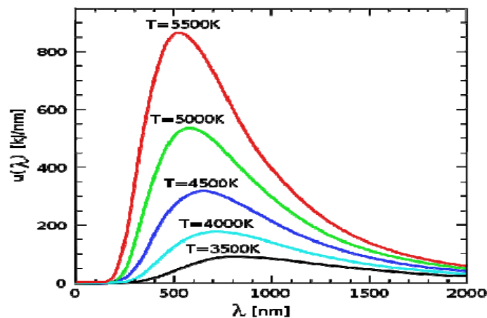
Fig.(10)Spectral irradiance for different black body temperature
